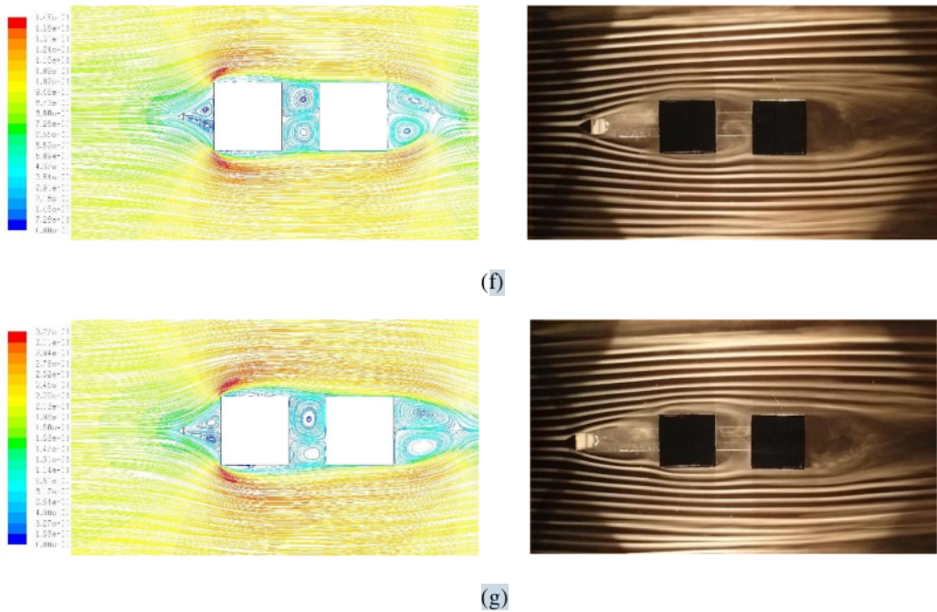
FIGURE 3. Comparison of computational and experimental velocity pathlines (a) M/D=0.00 , (b) M/D=0.05 , (c) M/D=0.15 , (d) M/D=0.25 , (e) M/D = 0.35 , (f) M/D=0.45 , (g) M/D=0.55
