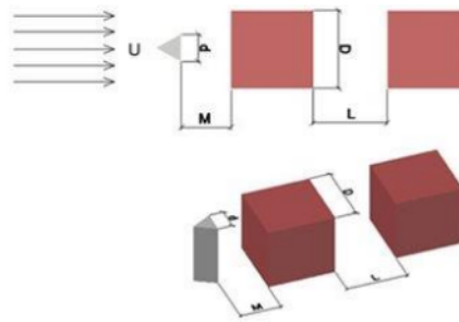
FIGURE 1. Test model
