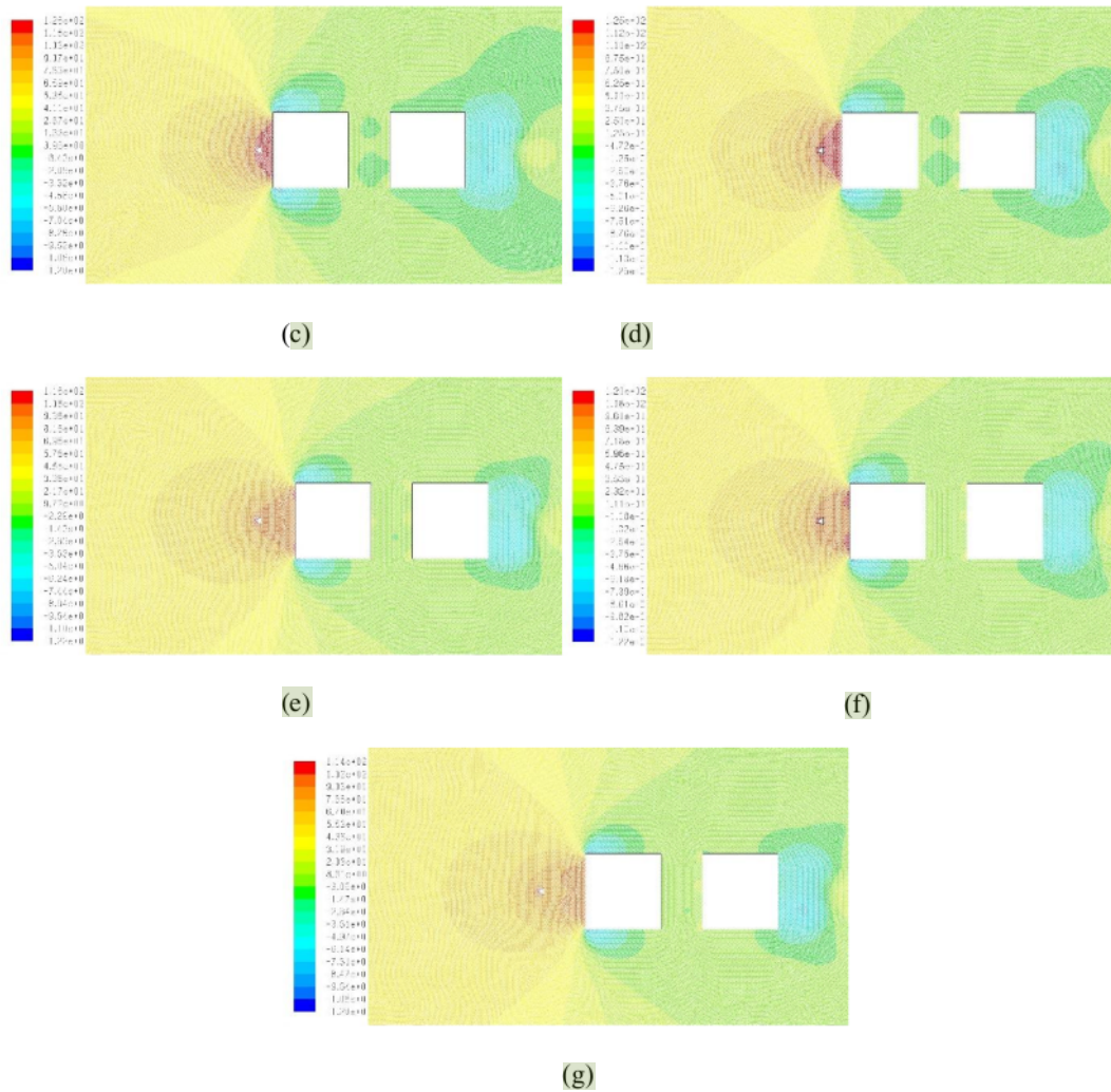
FIGURE 4. Comparison of pressure contours at various distance ratios (a) M/D=0.00 , (b) M/D=0.05 , (c) M/D=0.15 , (d) M/D=0.25 , (e) M/D=0.35 , (f) M/D=0.45 , (g) M/D=0.55
